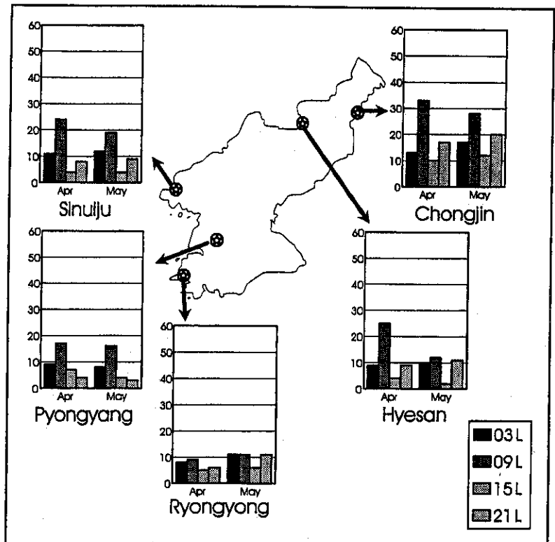
Figure 3-3. Spring Percent Frequencies of Visibilities Below
