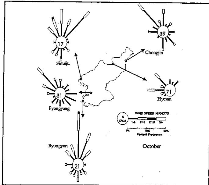
Figure 5-1. October Wind Roses.
