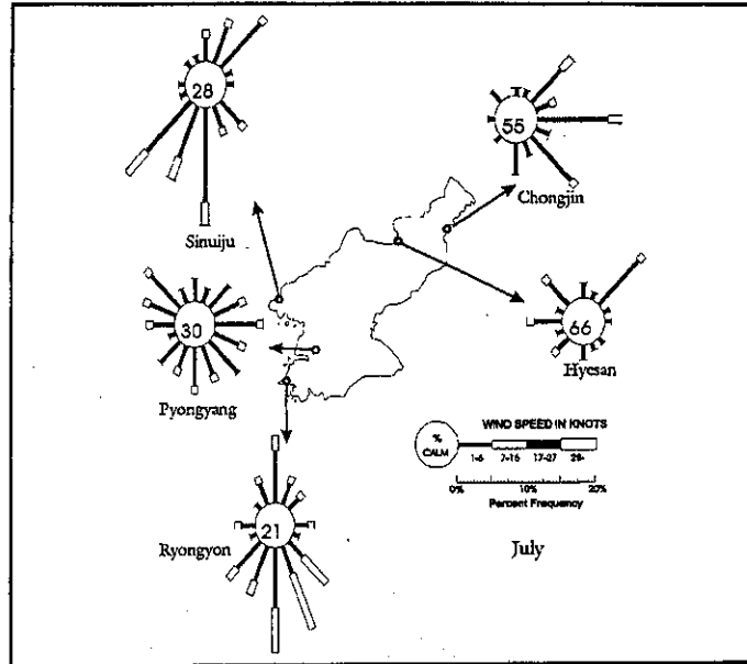
Figure 4-1. July Wind Roses.
