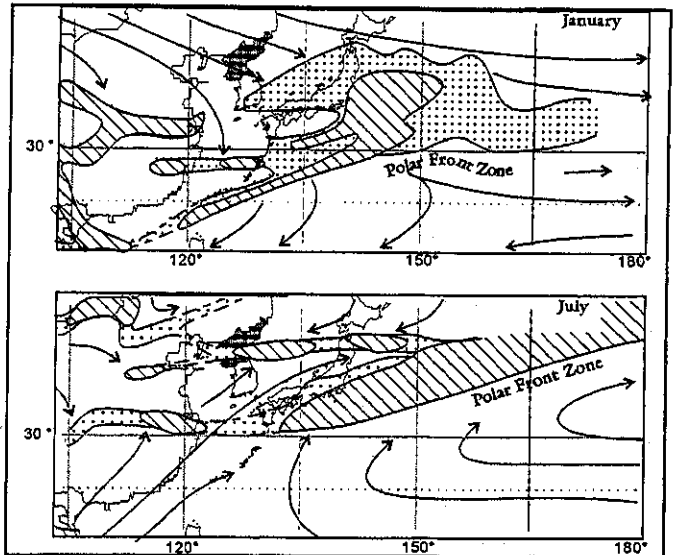
Figure 2-6. Polar Frontal Zones around North Korea. Arrows indicate steady wind direction.
