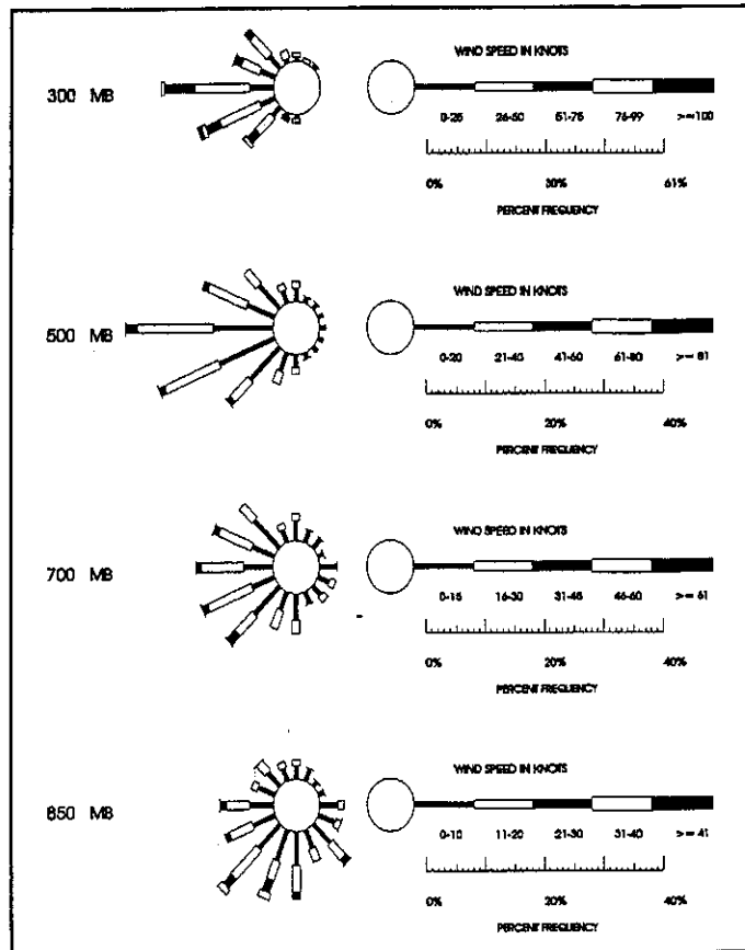
Figure 4-2. July Upper-Air Wind Roses for Pyongyang.
