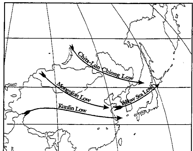
Figure 2-8. Storm Tracks Affecting North Korea.
