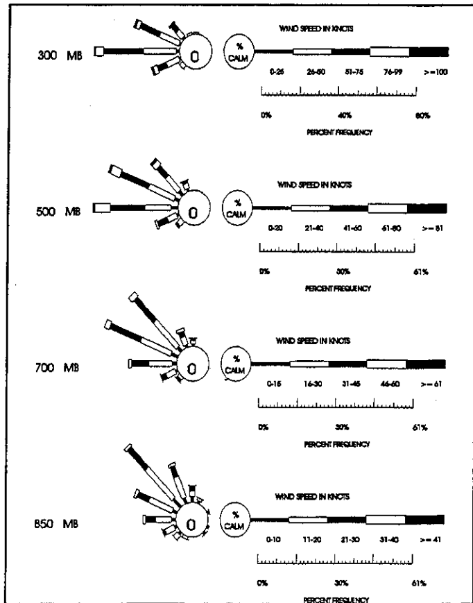
Figure 6-2. January Upper-Air Wind Roses for Pyongyang.
