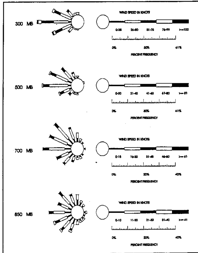
Figure 3-2. April Upper-Air Wind Roses.
