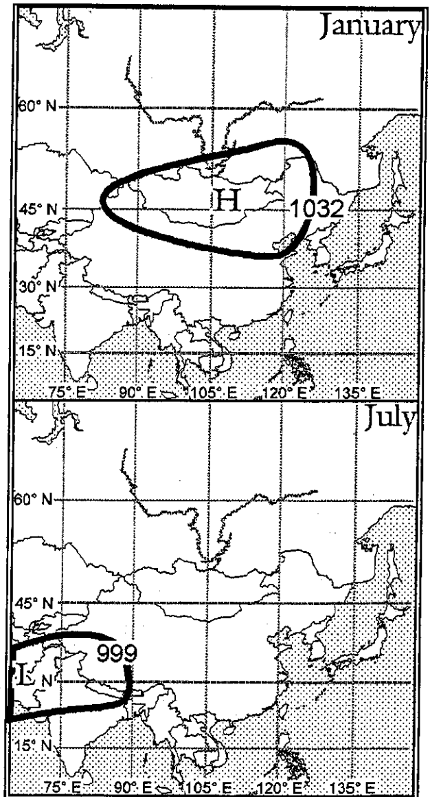
Figure 2-4. Major Continental Pressure Features. Top, Asiatic High; bottom, Asiatic Low.
