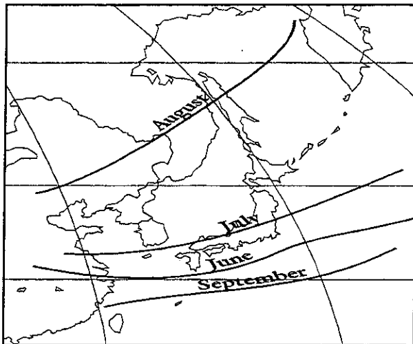
Figure 2-7. Summer Frontal Positions.
