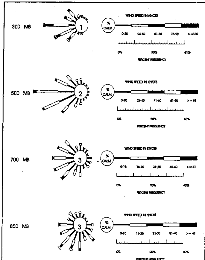
Figure 5-2. October Upper-Air Wind Roses for Pyongyang.
