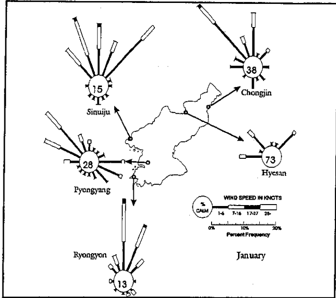
Figure 6-1. January Wind Roses.
