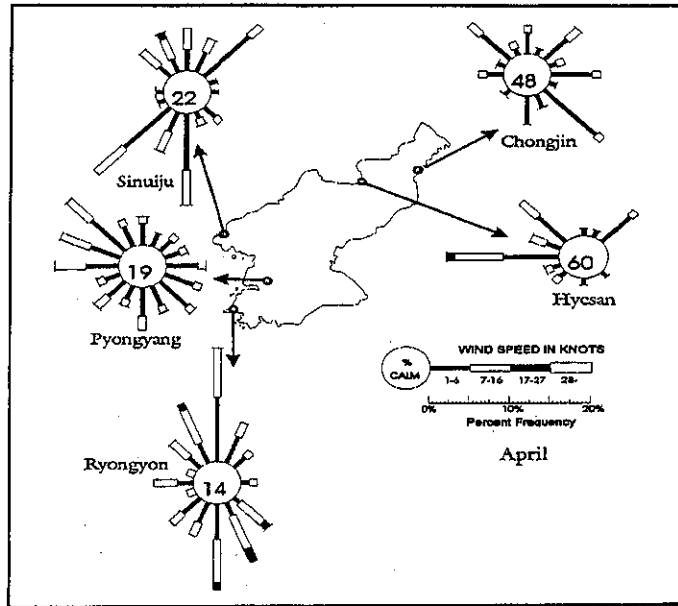
Figure 3-1. April Wind Roses.
