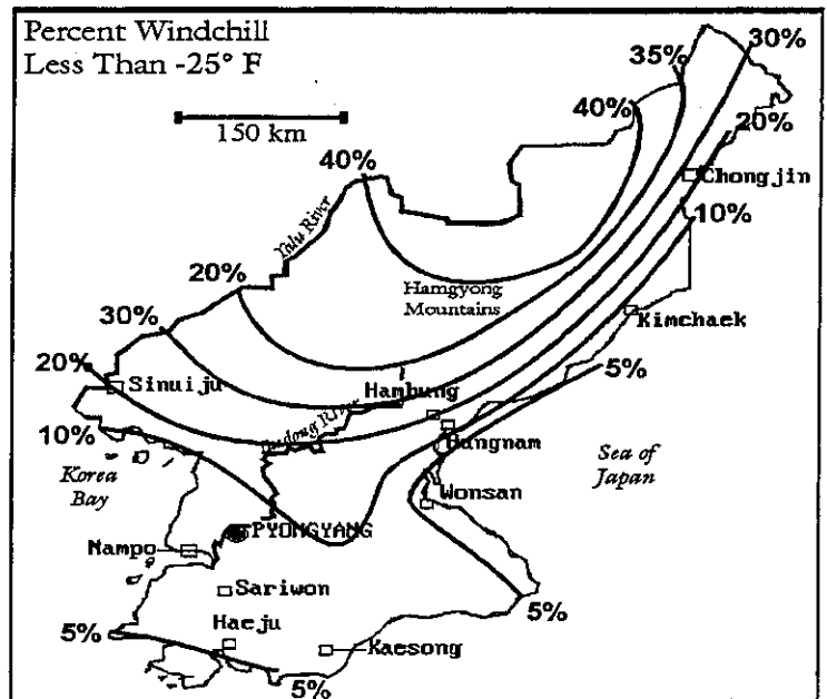
Figure 6-6. January Percent Frequencies of Windchills Below -25° F.
