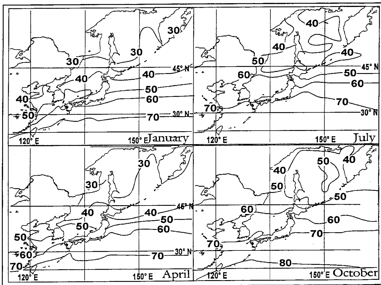
Figure 2-1. Mean Sea-Surface Temperatures.
