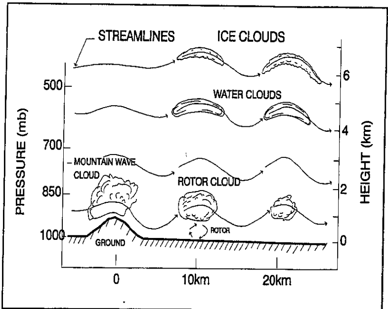
Figure 2-15 Fully Developed Lee Wave System (after Wallace and Hobbs, 1977).
